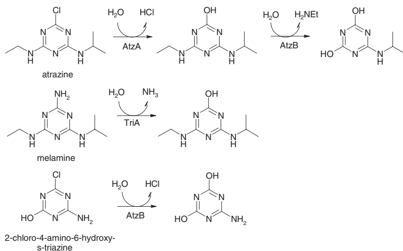
Fig. 5. Degradation of atrazine by AtzA and AtzB. These hydrolases both are members of the amidohydrolase superfamily. AtzA is highly similar to TriA, the enzyme that deaminates the amino analogue of atrazine called melamine. There are only nine substitutions and a short evolutionary pathway may be involved in adaptation of TriA to atrazine (Seffernick et al. , 2001). AtzB catalyses the second step in atrazine degradation, which is a deamination reaction, but it can also catalyse a dechlorination reaction with the atrazine soil metabolite 2-chloro-4,6-diamino-s-triazine to yield ammelide (Boundy-Mills et al. , 1997). These observations suggest that dechlorination and deamination activities are evolutionarily closely related.
