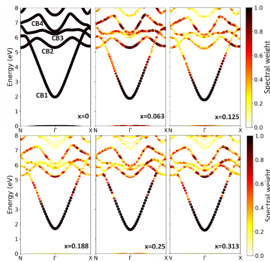
Figure 1: Band structures of \text{Ga}_2\text{O}_3 alloys (see ref. 2)
