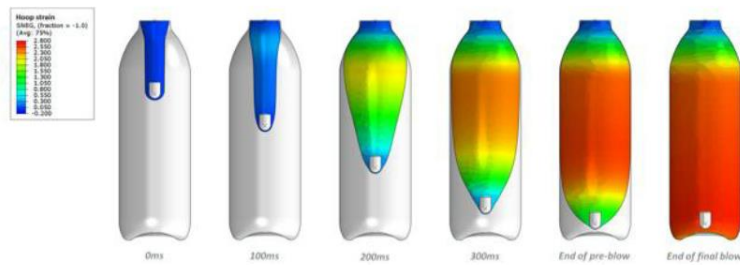
Figure 1: FEA simulation of stretch blow moulding
